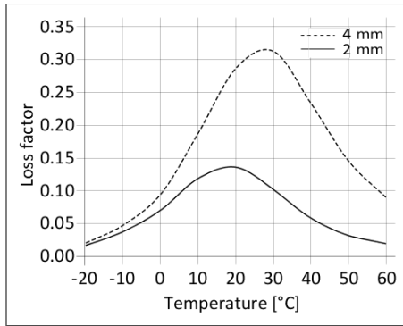
Diagram 1: Loss factor SikaDamp®-110 at 200 Hz
